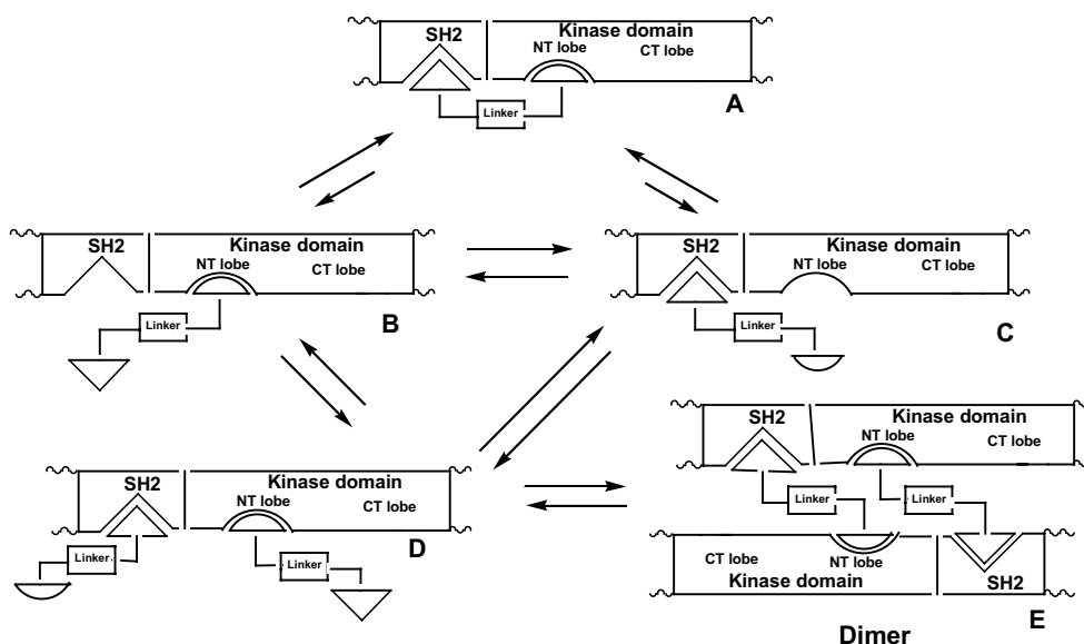
Figure 4. Possible mechanisms for the activity of ATP-phosphopeptide conjugates.
