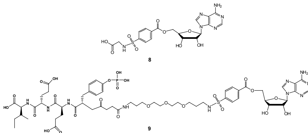
Figure 3. Chemical structures for 4-(carboxymethylsulfamoyl)benzoyladenosine ( 8 ) and synthesized 4-(sulfamoyl)benzoyladenosine-pYEEI (SBA-pYEEI) conjugate ( 9 ) as compounds with no binding affinity to ATP-binding site.
