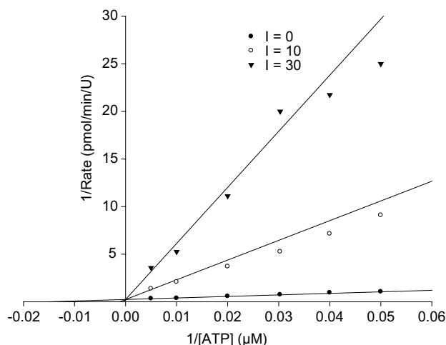
Figure 5. Pattern of inhibition of Src by compound 5 ; Lineweaver–Burk plot of 1/V versus 1/ATP with varying concentration of 5 shows linear competitive inhibition ( K_i = 1.7 \mu M ).
