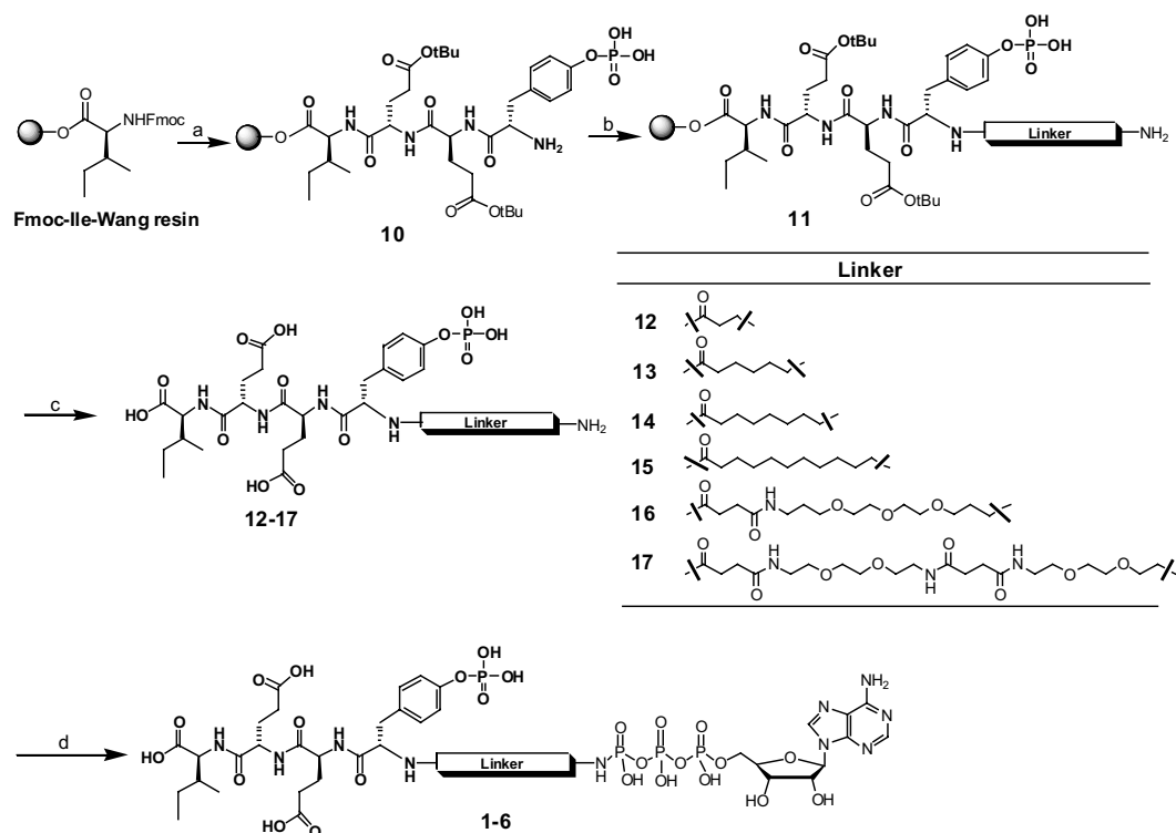
Scheme 1. General synthetic strategy for the preparation of ATP-phosphopeptide conjugates ( 1–6 ). Reagents and conditions: (a) Fmoc-peptide chemistry: Fmoc-AA-OH, HBTU, NMM, piperidine, DMF; (b) (i) FmocNH(A)COOH, (ii) piperidine/DMF (1:4) or (i) succinic anhydride, NMM, DMF, (ii) 3,6,9-trioxa-1,13-diamine, HBTU, NMM, DMF or (i) succinic anhydride, NMM, DMF, (ii) 1,8-diamino-3,6-dioxaoctane, HBTU, NMM, DMF, (iii) succinic anhydride, NMM, DMF, (iv) 1,8-diamino-3,6-dioxaoctane, HBTU, NMM, DMF; (c) TFA, anisole, water; (d) ATP, CMD-CDI, water, pH = 7.
