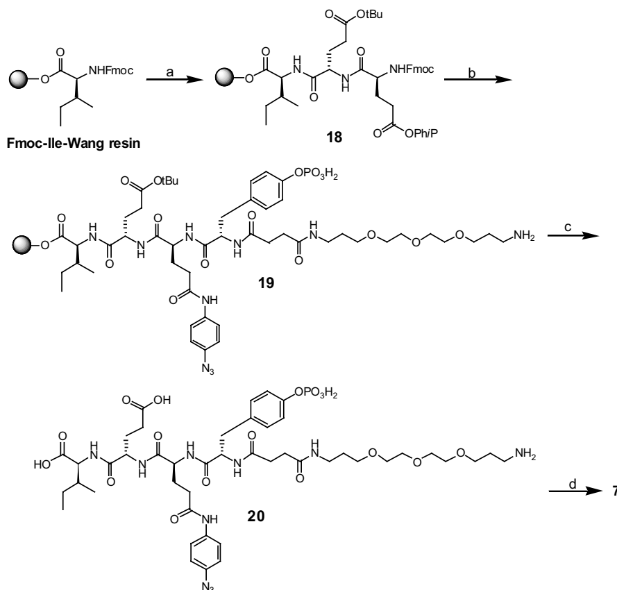
Scheme 2. Synthesis of diazido ATP-phosphopeptide conjugate 7 . Reagents and conditions: (a) Fmoc-peptide chemistry; (b) (i) TFA/DCM/TIPS (1:94:5), (ii) p -azidoaniline, HBTU, NMM, DMF, (iii) piperidine 20%/DMF, (iv) Fmoc-Tyr(PO 3 H 2 )-OH, HBTU, NMM, DMF; (v) piperidine 20%/DMF, (vi) succinic anhydride, NMM, DMF, (vii) 4,7,10-trioxa-1,13-tridecanediamine, HBTU, NMM, DMF; (c) TFA/DCM; (d) 8-azidoATP, CDI-CMD, water, 5 h, rt.
