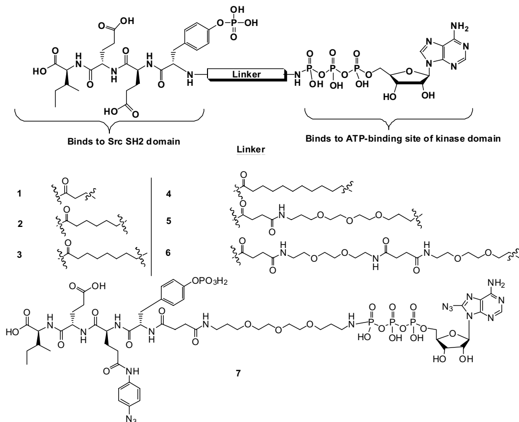
Figure 1. Synthesized ATP-phosphopeptide conjugates (1–7) as Src kinase inhibitors targeting the Src SH2 domain and ATP-binding site.
