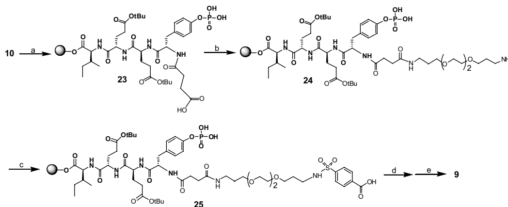
Scheme 4. Synthesis of SBA-Linker-pYEEI derivative 9 . Reagents and conditions: (a) succinic anhydride, DIEA, HBTU, DMF; (b) 4,7,10-trioxal,1,13-tridecanediamine, DIEA, HBTU, DMF; (c) p -chlorosulfonylbenzoic acid, DMF, pyridine; (d) (i) DCC, DMAP, DMF/DCM (ii) 2',3'-O-isopropylideneadenosine, DMF; (e) TFA/DCM, EDT, H 2 O.
