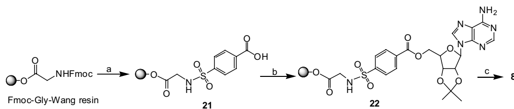
Scheme 3. Synthesis of 4-(carboxymethyl-sulfamoyl)-benzoyl adenosine ( 8 ). Reagents and conditions: (a) (i) piperidine/DMF (1:4), (ii) 4-(chlorosulfonyl)benzoic acid, pyridine/DMF; (b) 2',3'-O-isopropylideneadenosine, DCC, DMAP, DMF/DCM; (c) TFA/DCM.
